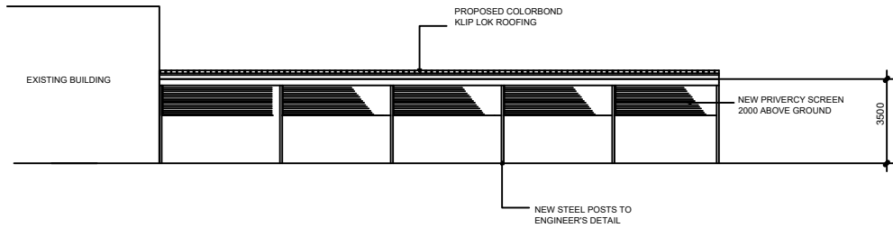
NORTH ELEVATION
